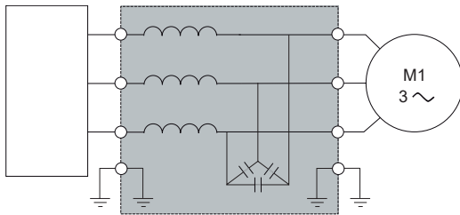
Sinus filter
